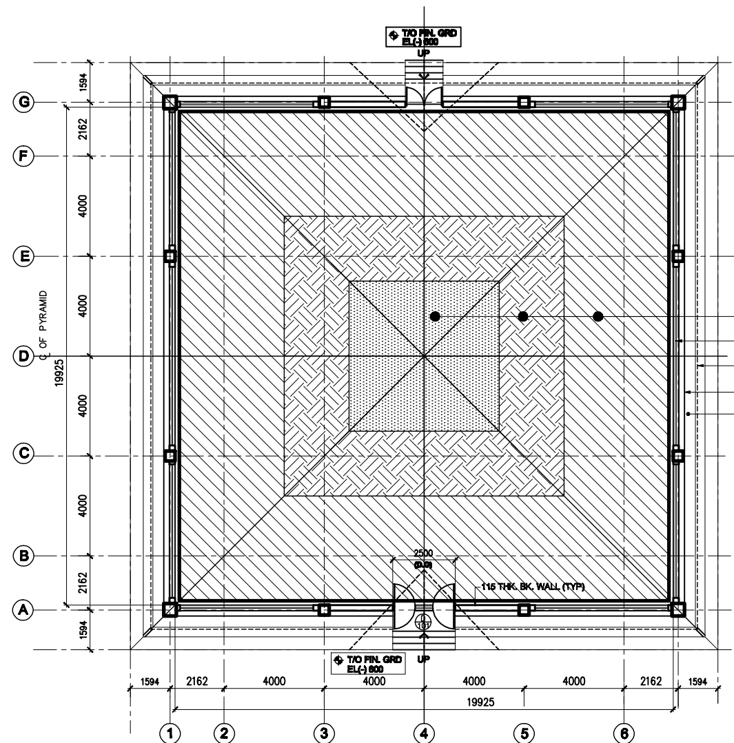
REFLECTED FALSE CEILING PLAN OF PYRAMID
